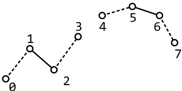
GL_LINES_ADJACENCY
