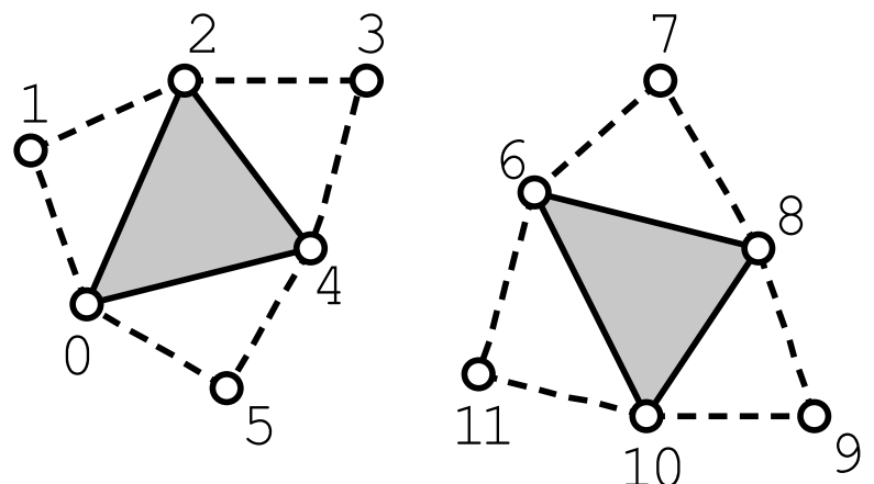
GL_TRIANGLES_ADJACENCY
