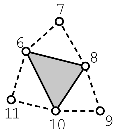
GL_TRIANGLES_ADJACENCY
