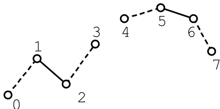
GL_LINES_ADJACENCY
