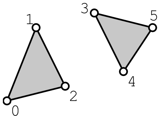
GL_TRIANGLES
